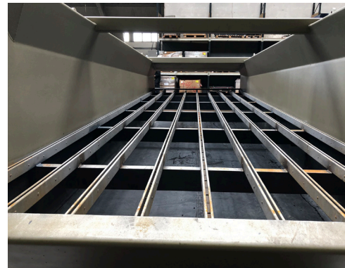
Rubber Lining Project : T-REX60 thickness 20 mm, ± 30 square metres
